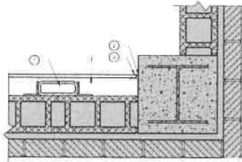
2 PLAN DETAIL 1/12" = 1'-0"
