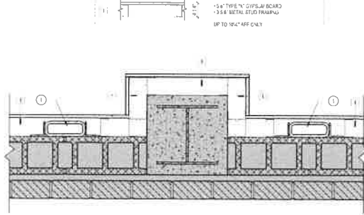
1 PLAN DETAIL 1/12" = 1'-0"
